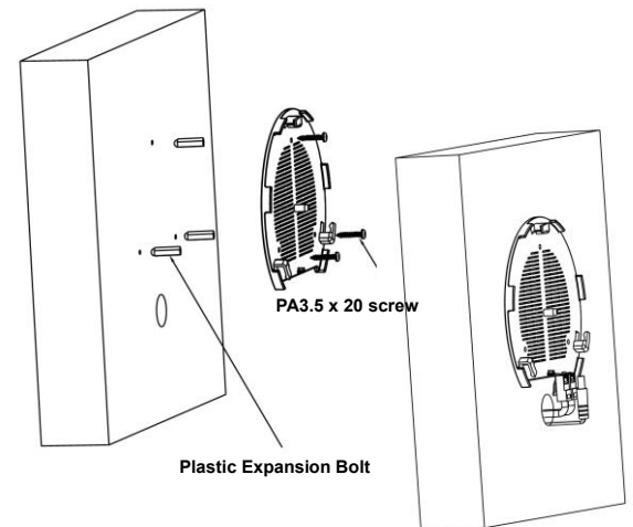
Figure 3: Wall Mount – Steps 1 & 2
