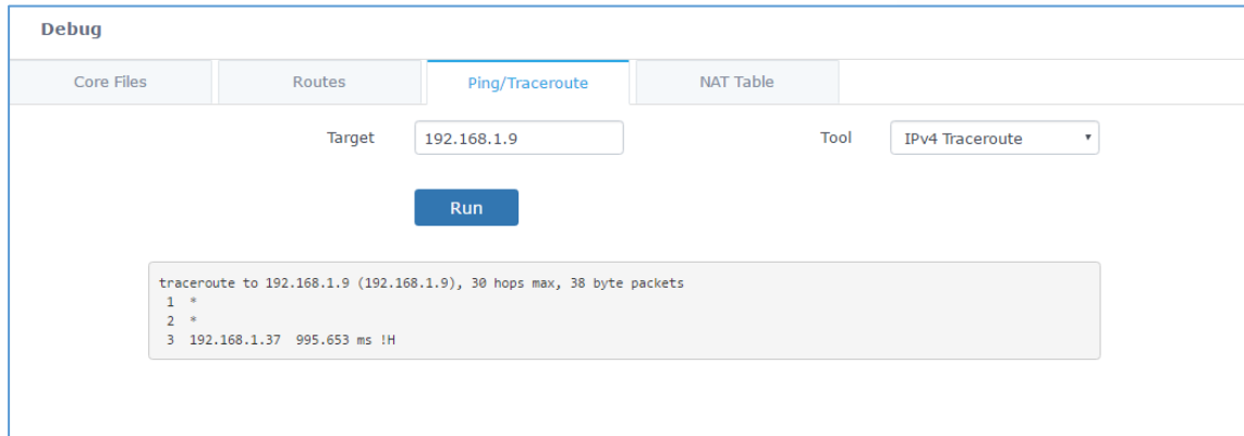
Figure 35: IP Traceroute
