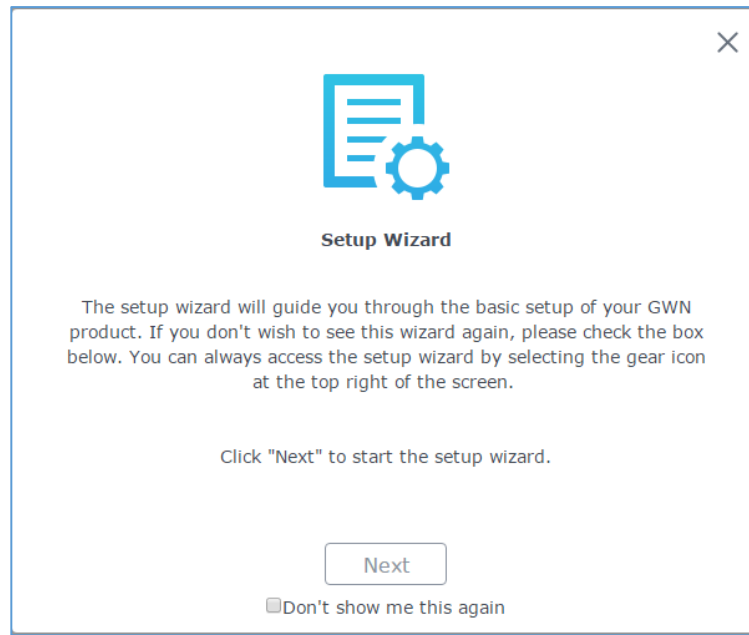
Figure 20: Setup Wizard
