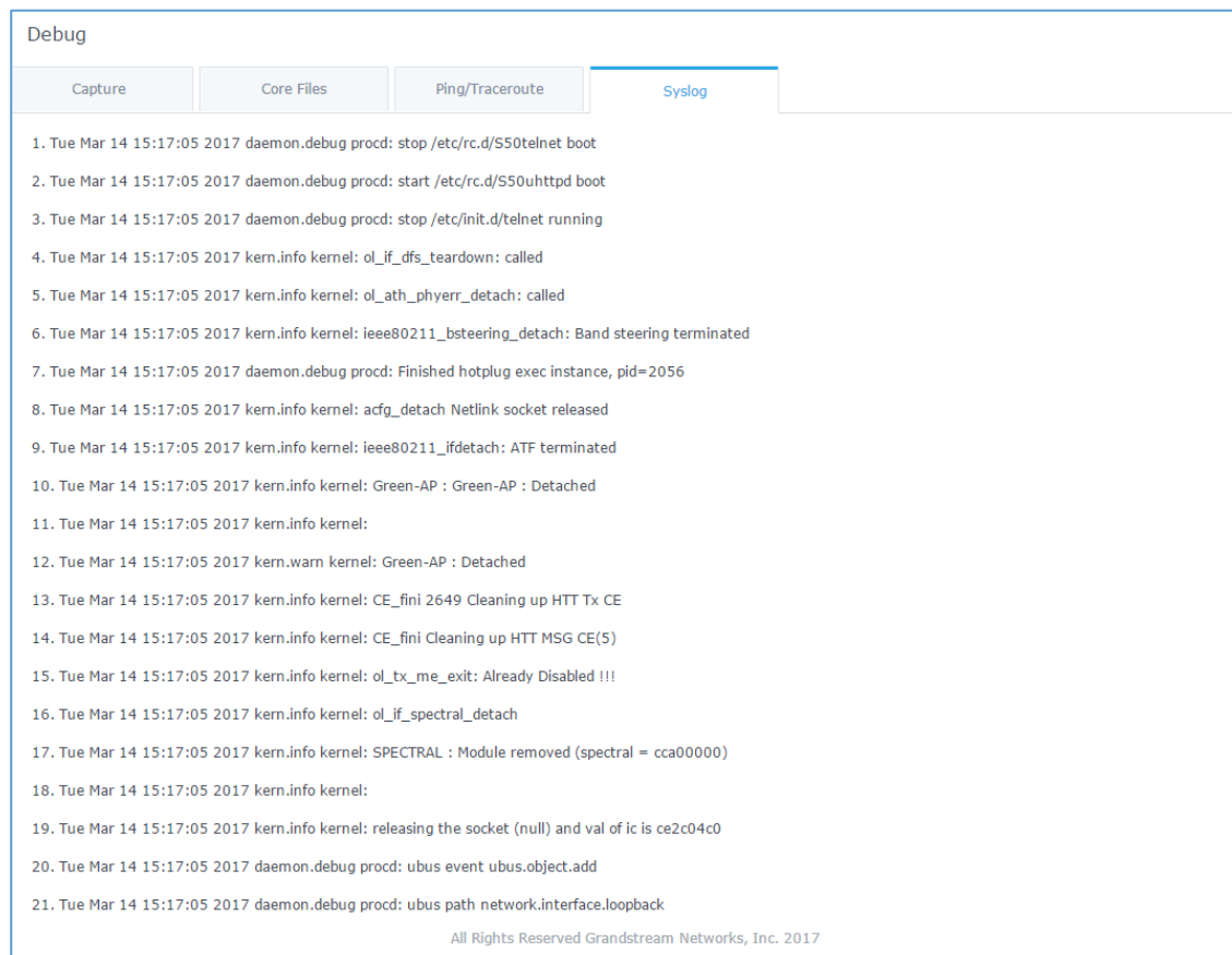
Figure 36: Syslog
