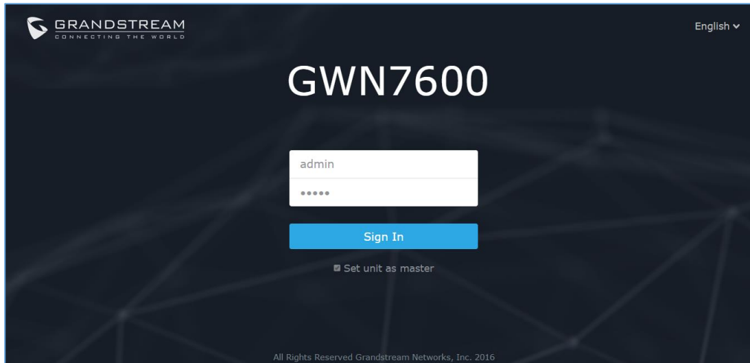
Figure 19: Login Page
