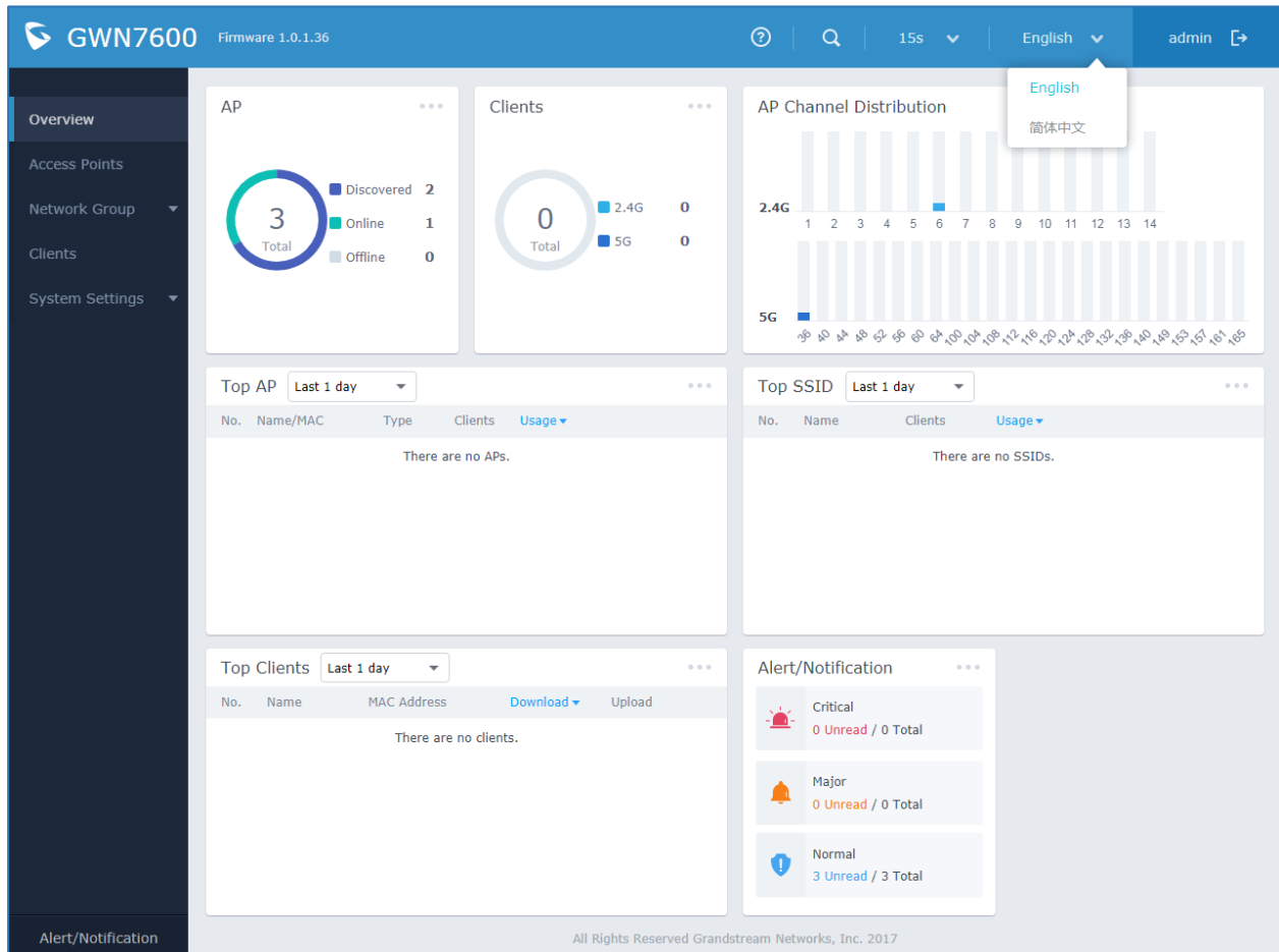
Figure 16: GWN7600's Dashboard
