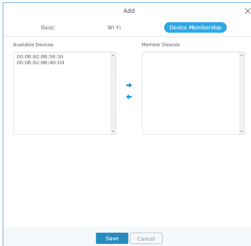
Figure 26: Device Membership
