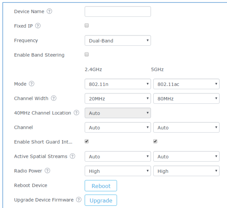
Figure 38: Device Configuration
