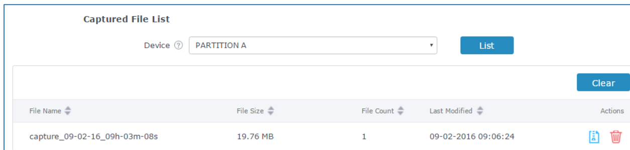
Figure 33: Capture Files
