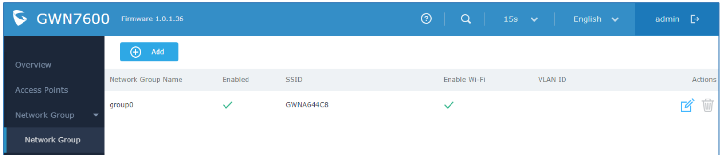
Figure 24: Network Group
