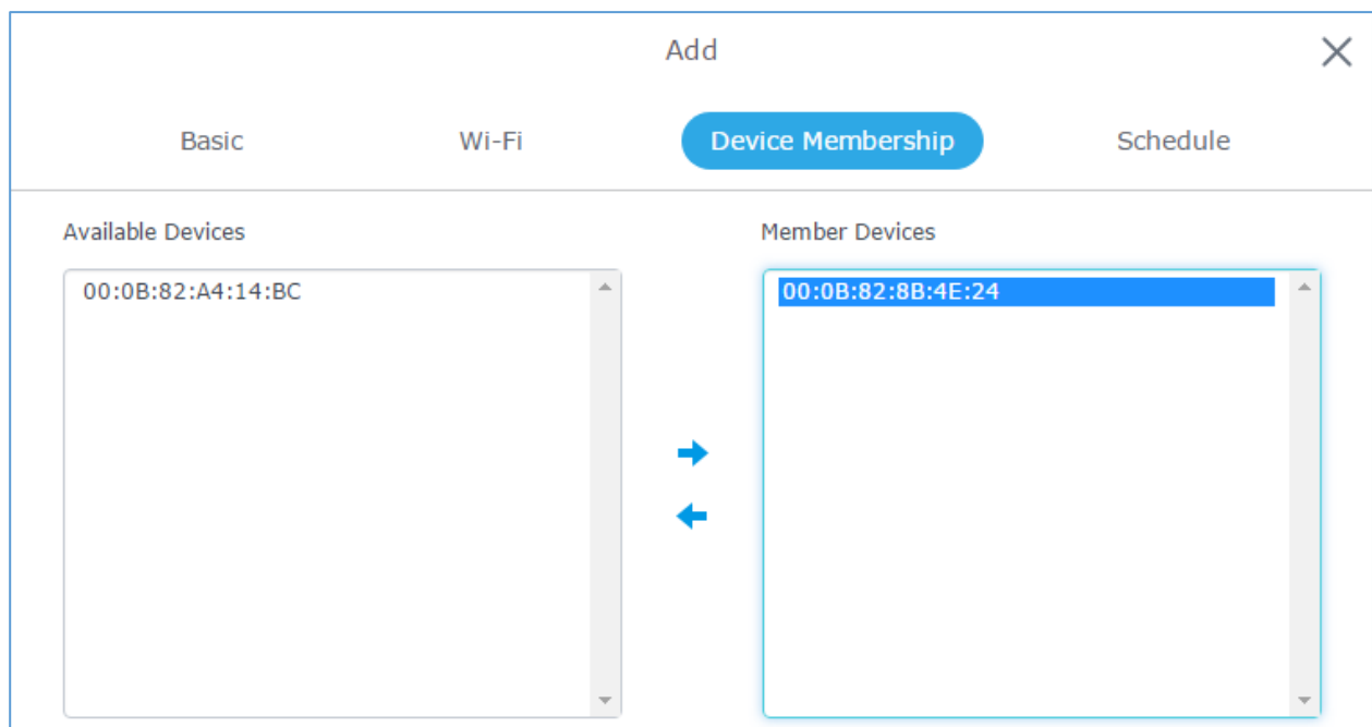
Figure 27: Device Membership
